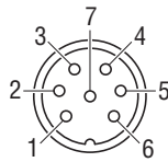
Front side molded 7P Male connector
